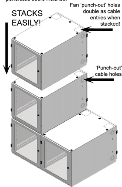
RCSC 12U, 36" deep cabinet shown here with optional perforated doors installed.
